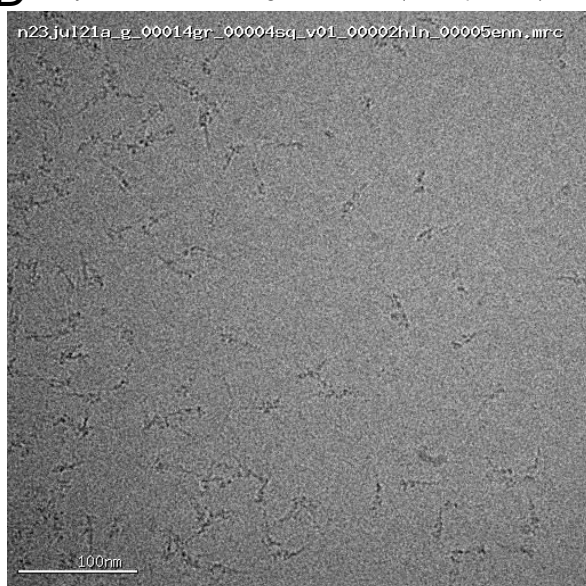
D Cryo-EM kinesin-1 from grids at NCATT (33 nm particles)
