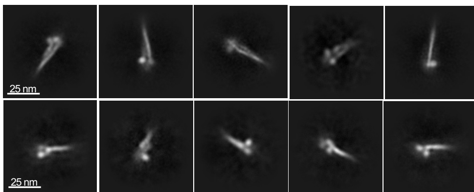
E Cryo-EM kinesin-1 2D-class averages resulting from NCATT Krios
