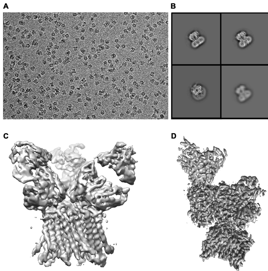
Figure 1. Representative preliminary cryo-EM data. (A-B) Micrograph and 2D class averages of an ion channel complex. (C) Initial 3D reconstruction of an ion channel complex at \sim 4.0 Å resolution. (D) Initial 3D reconstruction of a membrane enzyme at \sim 3.5 Å resolution.
