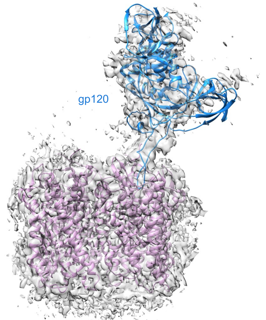
CXCR4 tetramer
