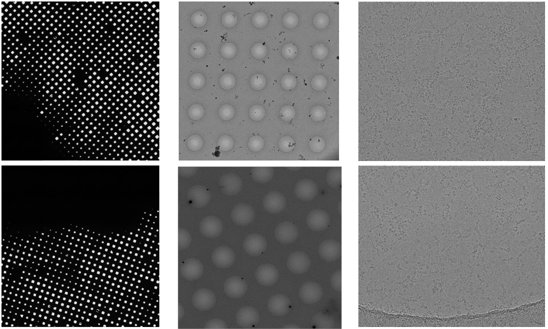
Figure 2. Representative low, medium, and high mag images of two screened grids of the GSDME/Caspase-3 complex. Samples were prepared on Quantifoil R1.2/1.3 (Cu 300mesh) holey carbon grids.
