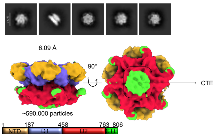
Figure 1. Screening and cryo collection of p97 in a Glacios microscope. A) Representative micrograph of a Glacios screening of p97 in the presence of 1.2 mM DDM using Quantifoil 1.2/1.3 Au 300 mesh grids. The grids are currently stored at the NCCAT. B) 2D classification of p97 Glacios collection in the presence of 1.2 mM DDM using Quantifoil 1.2/1.3 Au 300 mesh grids. The 2D classification shows sufficient orientations for Krios acquisition. The 6.09 Å 3D reconstruction reveals the presence of the CTE (lime green).
