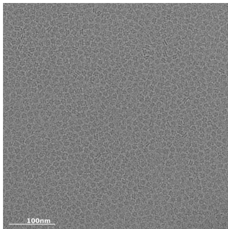
Figure 1. Screening and cryo collection of p97 in a Glacios microscope. A) Representative micrograph of a Glacios screening of p97 in the presence of 1.2 mM DDM using Quantifoil 1.2/1.3 Au 300 mesh grids. The grids are currently stored at the NCCAT. B) 2D classification of p97 Glacios collection in the presence of 1.2 mM DDM using Quantifoil 1.2/1.3 Au 300 mesh grids. The 2D classification shows sufficient orientations for Krios acquisition. The 6.09 Å 3D reconstruction reveals the presence of the CTE (lime green).
