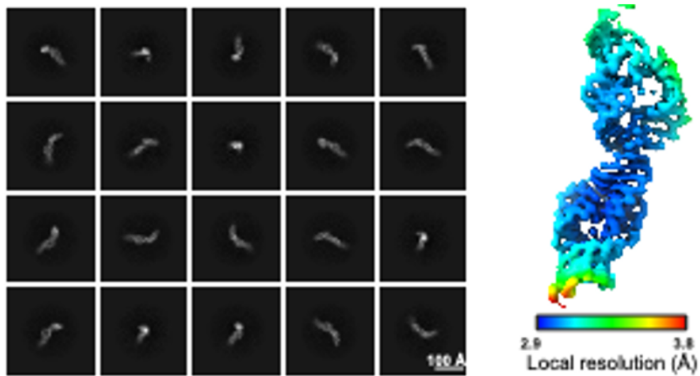
Figure 1. 2D class averages and 3D reconstruction of the first RNA device (3 Å resolution). Other RNA devices in our pipeline are expected to yield similar results, whose various structures will provide critical mechanistic insight.
