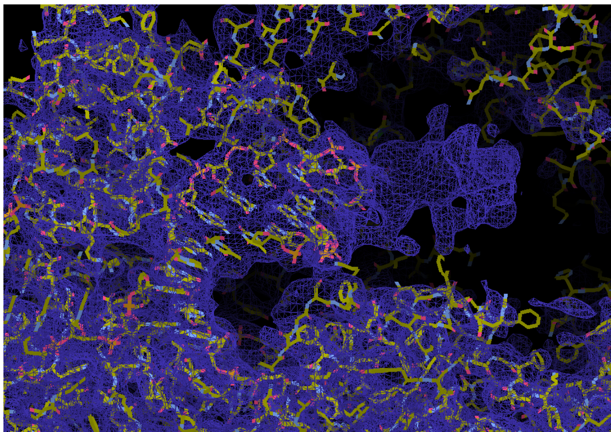
Figure 1. Cas12a fitted into calculated Cryo-EM SPA map.
