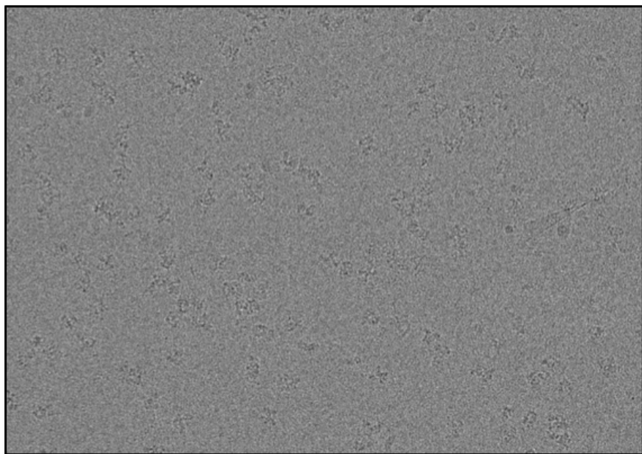
Figure 1. A) Chromatogram of the biochemically reconstituted and purified destruction complex, with major peak representing the "full-complex." B) SDS-PAGE of pooled fractions of the gel-filtered complex. C) Representative micrograph collected on Titan Krios / K3 at PNCC. D) 2D classification (Cryosparc) from dataset in (C).
