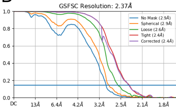
Figure 2: Preliminary structure of nanodisc reconstituted AE1. (A) Representative micrograph. (B) 2.37 Å refinement of AE1, with one monomer in the inward facing, and one in the outward facing state. (C) Representative 2D class averages. (D) FSC of the reconstruction in (B).
