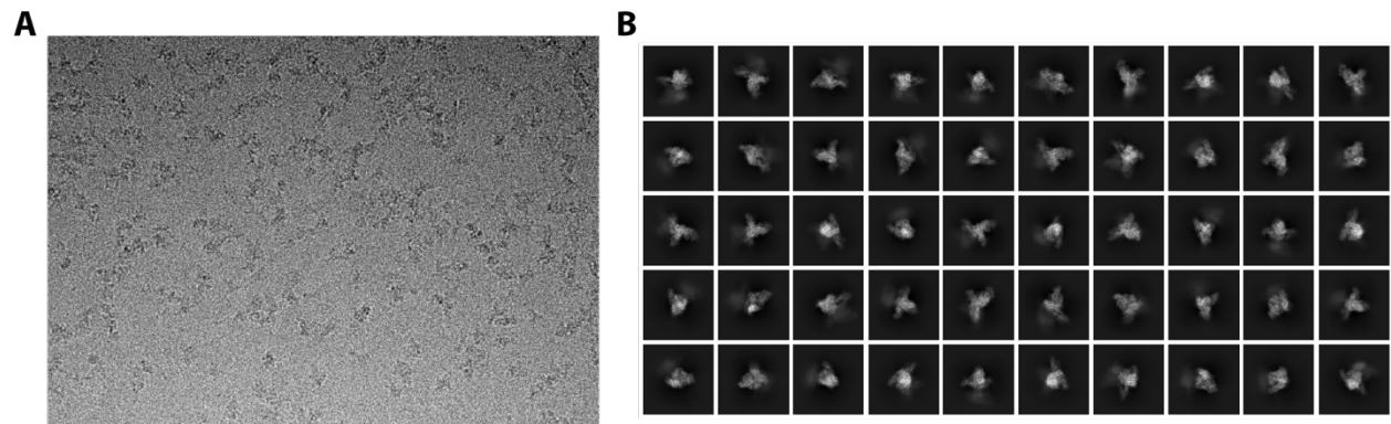
Figure 1. Preliminary cryo-EM characterization of coronavirus RTC-RNA complex. (A) A representative cryo-EM image of the SARS-CoV-2 RTC-RNA complex imaged on a Glacios 200 kV cryo-TEM. (B) Representative 2D classes generated from a preliminary SARS-CoV-2 RTC-RNA complex cryo-EM dataset collected on a Glacios 200 kV cryo-TEM.
