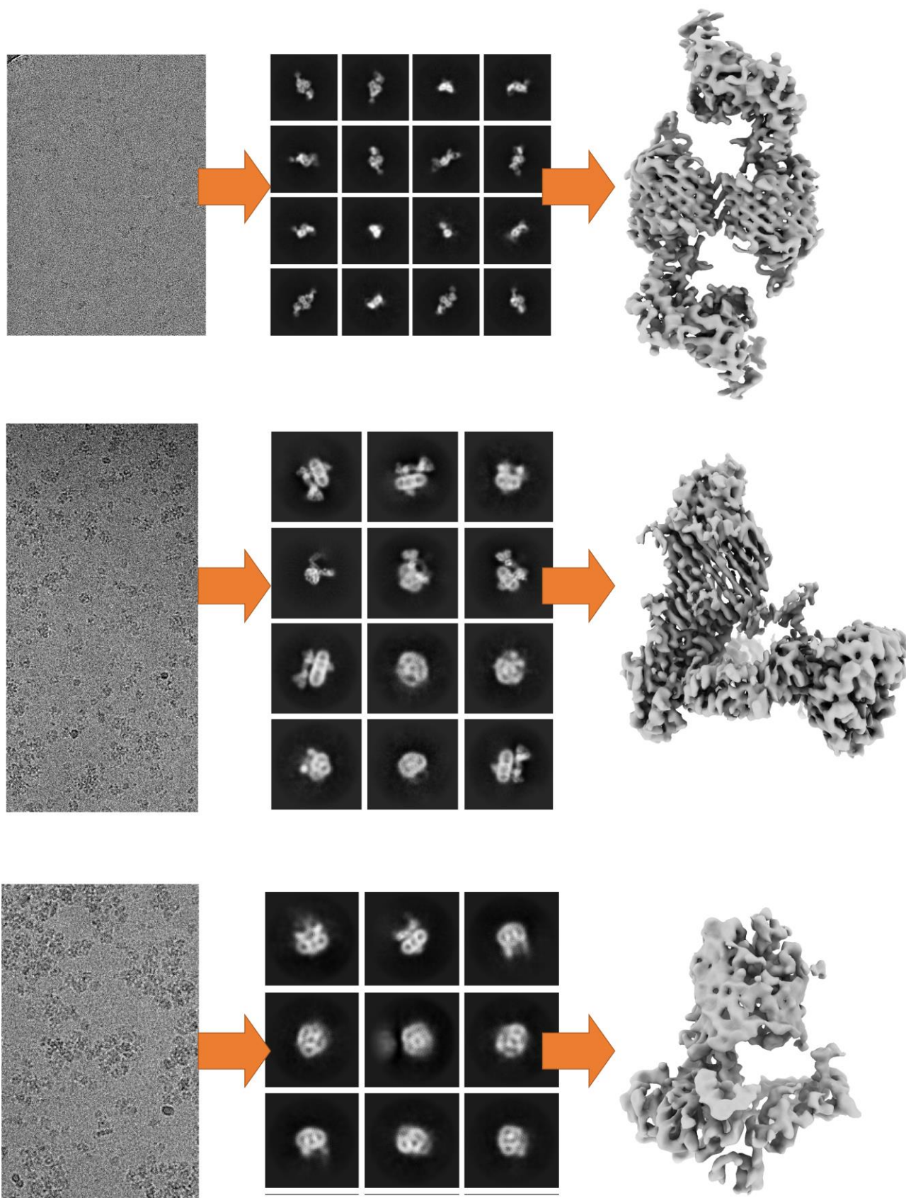
Fig. 1. Preliminary Cryo-EM Results. Top , FnBamA/Fab9 complex (150 kDa) showing a micrograph, 2D class averages, and the current state of the reconstruction. Middle , BAM \Delta BamC (175 kDa) complex showing a micrograph, 2D class averages, and the current state of the reconstruction. Bottom , NgBAM complex (175 kDa) showing a micrograph, 2D class averages, and the current state of the reconstruction.
