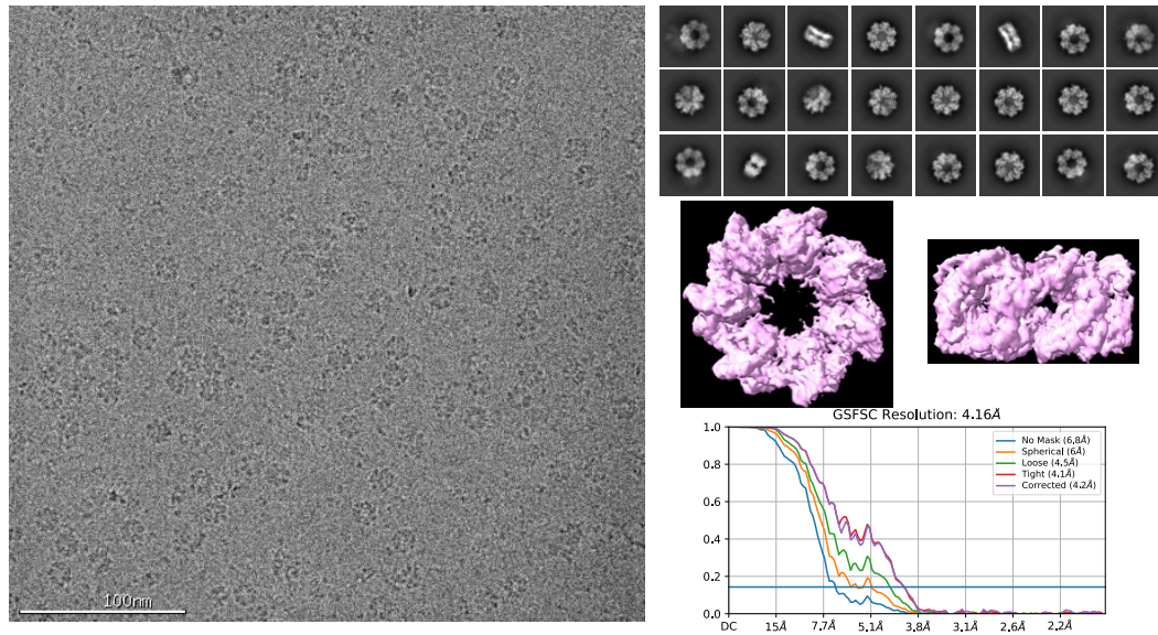
Figure CryoEM analysis of a mHsp60 mutant. Left, A representative micrograph of a mHsp60 mutant collected using a Krios EM microscope. Right, 2D class averages (top panel); top and side views of the 3D reconstruction (middle panel); reconstruction resolution (bottom panel). The 3D reconstruction is from 161,686 particles from 3,979 micrographs.
