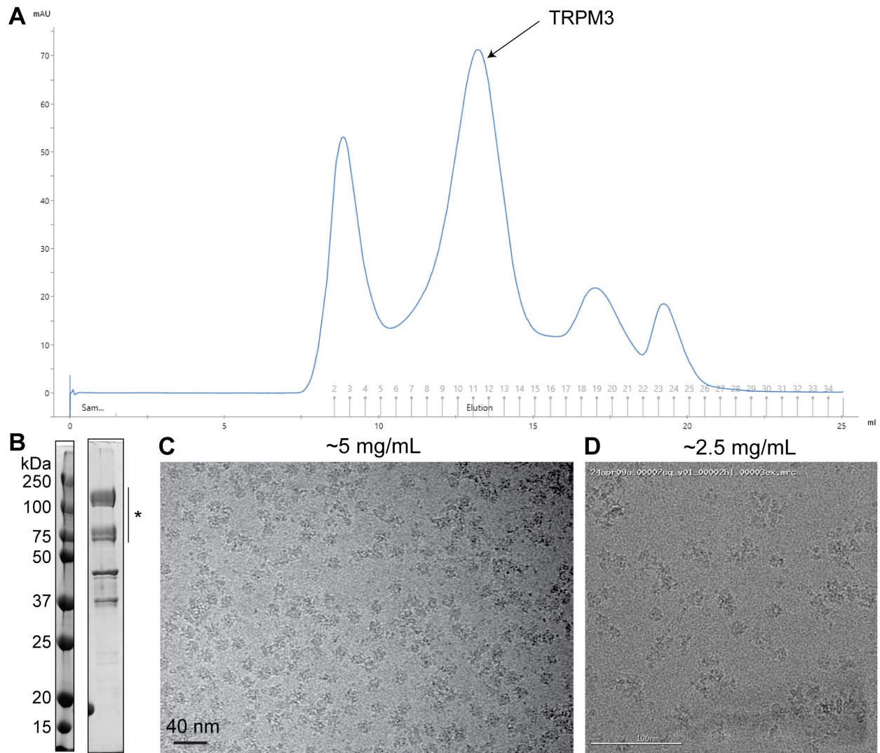
Figure 1. Preliminary data of TRPM3 sample for cryo-EM screening. (A) Gel-filtration profile of TRPM3. The peak fractions (fractions 9-12) were pooled and concentrated to ~5 mg/mL. (B) SDS-PAGE of the cryo-EM sample. *: TRPM3 (2 isoforms). (C) A previous cryo-EM micrograph of TRPM3 at 5 mg/mL collected on a Titan Krios equipped with K3 camera and energy filter. (D) A recent cryo-EM micrograph of a similar TRP channel at 2.5 mg/mL screened on the SECM4 Krios with the Apollo camera.
