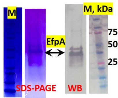
Figure 2. SDS-PAGE and western blotting (WB) of purified Mtb EfpA exporter.
