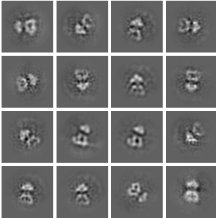
Representative 2D classes of MsbA, Apo state
