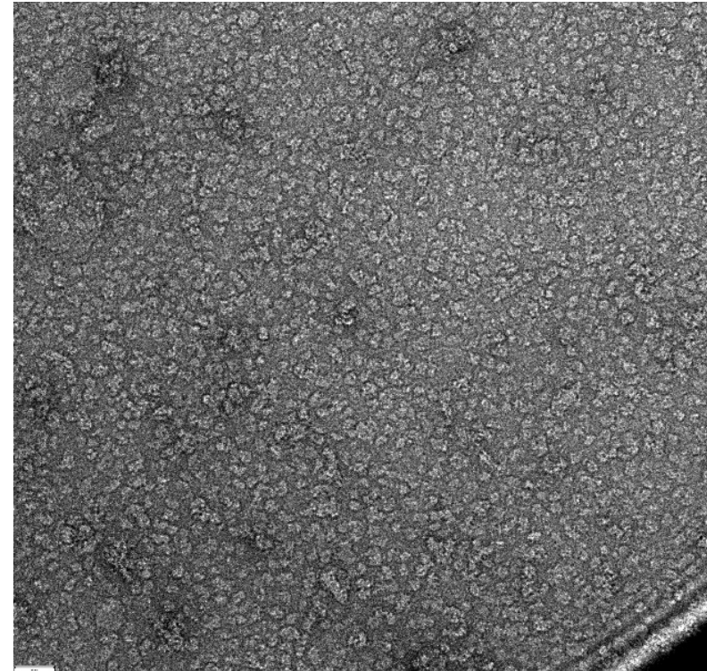
Negative-stain image of ABCB1 showing relative homogenous particles, Apo state
