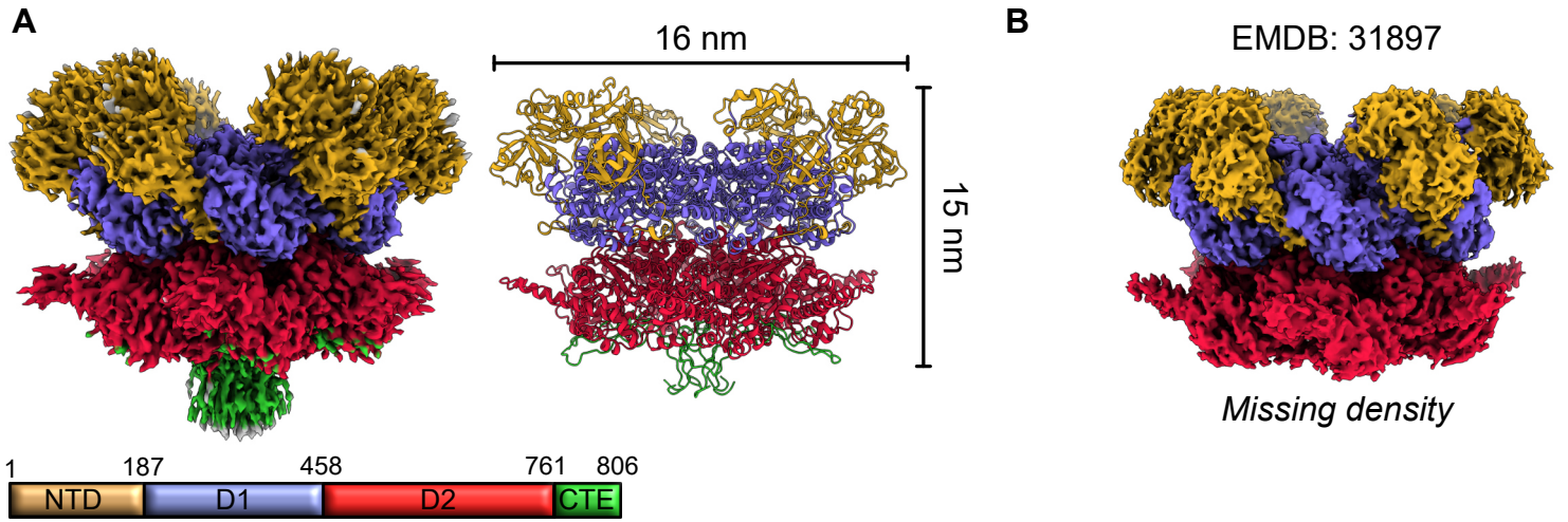
Figure 1. Our cryoEM studies of p97. A) Density map of p97 in the presence of 1.2 mM DDM at 3.5 Å and atomic reconstruction with all domains color-coded. B) Representative density map of p97 showing the missing density of the CTE (EMDB 31897) in the presence of detergent at sub-CMC.
