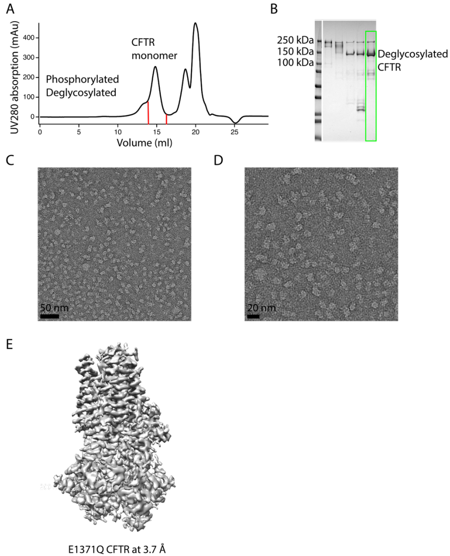
Figure 1. Protein purification and EM data of CFTR chloride channel. A. Size exclusion chromatography profile showing CFTR monomer can be readily purified in detergent. B. SDS-PAGE gel indicating the deglycosylated CFTR has a molecular weight at around 130 kDa. C and D. Negative staining images under different magnifications showing CFTR molecules separate well when in detergent. Different scale bars at the bottom of the image also indicate the right size of the protein. E. A high-resolution CFTR density map obtained using data collected at NCCAT.
