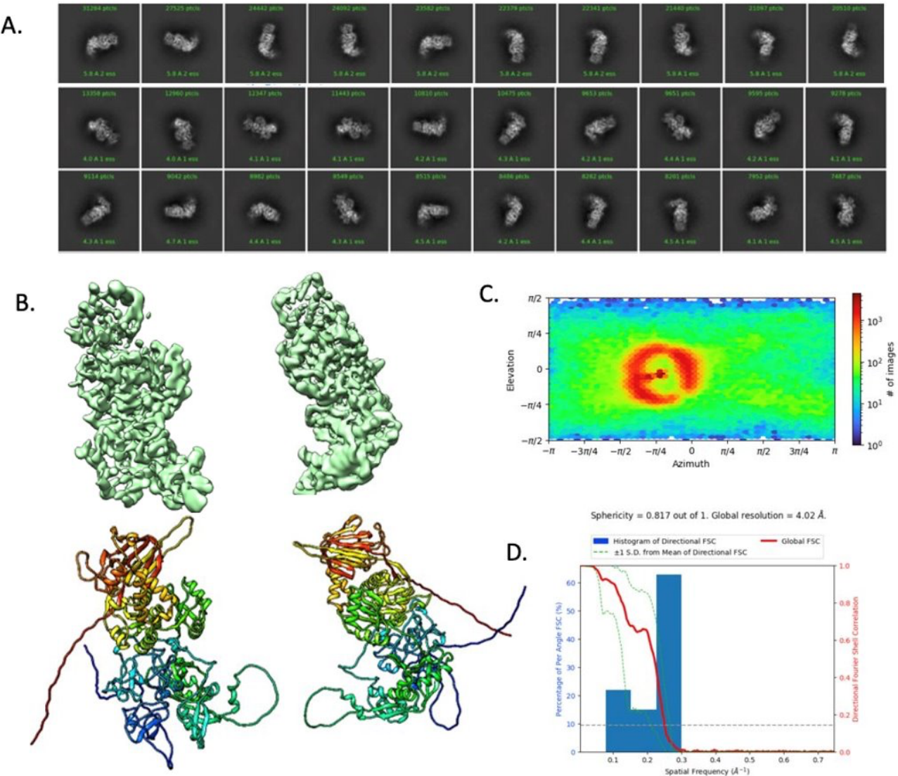
figure 2. cryoEM data processing of DGK \theta . A. Representative 2D class average. B. 3D reconstruction of DGK \theta compared to alphaFold prediction. C. View direction distribution D. 3DFSC of DGK \theta
