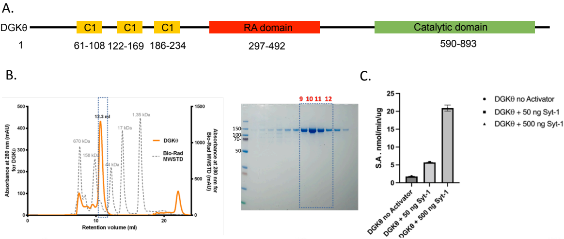
figure 1. A. Structure basis of the DGK \theta . B. Gel filtration profile and SDS-PAGE of DGK \theta . C. Kinase activity assays of DGK \theta with and without neuronal activator.
