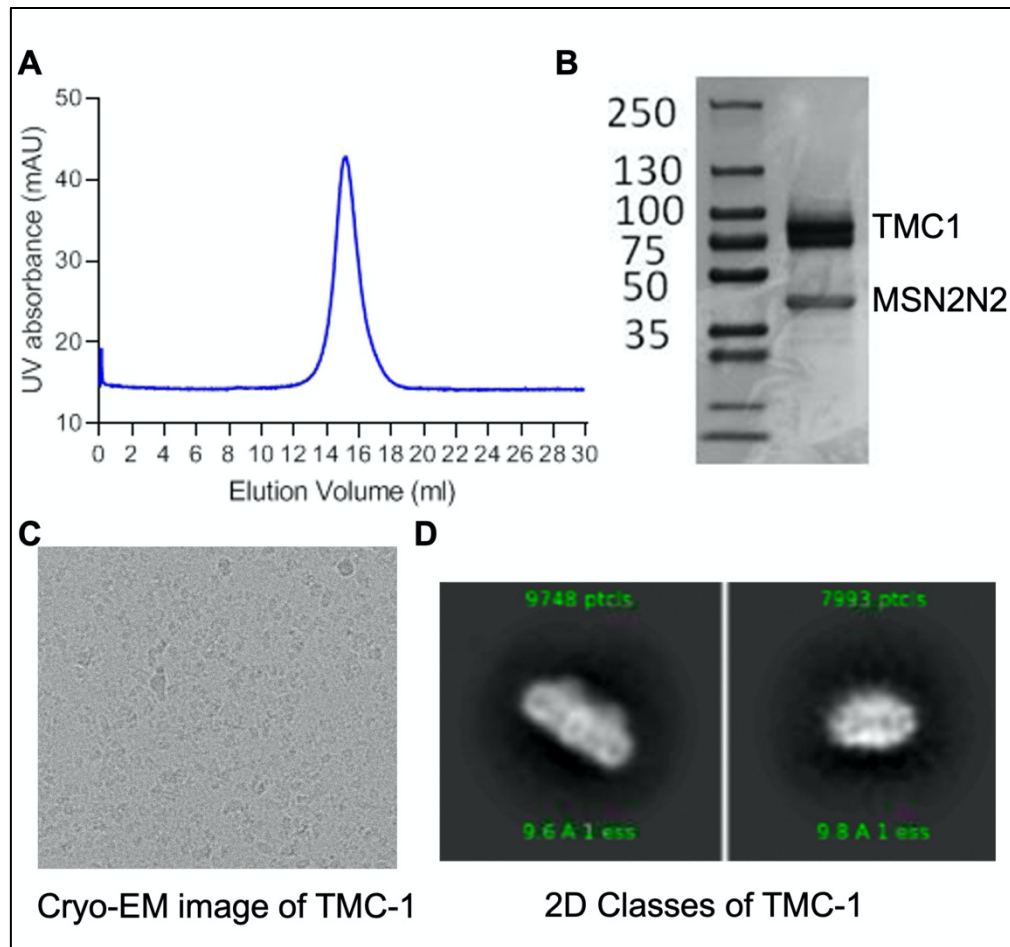
Fig. 1. Purification and EM analysis of TMC-1. A. The gel filtration profile of TMC-1 purification. B. SDS-PAGE gel of the purified TMC-1 in nanodiscs. C. a representative Cryo-EM image of TMC-1. D. Representative 2D classes of TMC-1.
