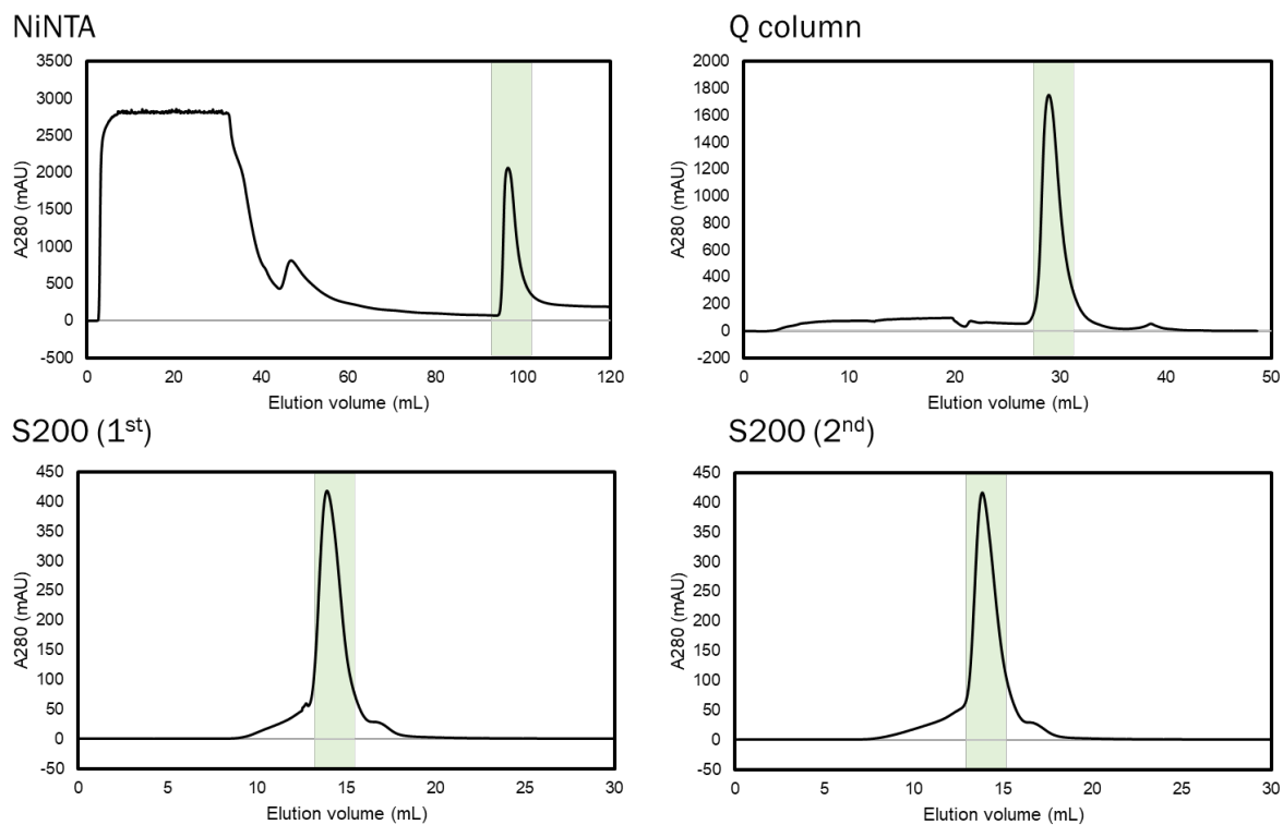
Figure S1. Chromatography of three-column strategy for purification of the SARS-CoV2 RdRp complexes.
