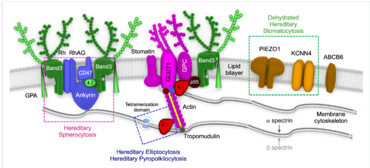
Figure 1 shows the primary functional components of the membrane structure of a red blood cell.
