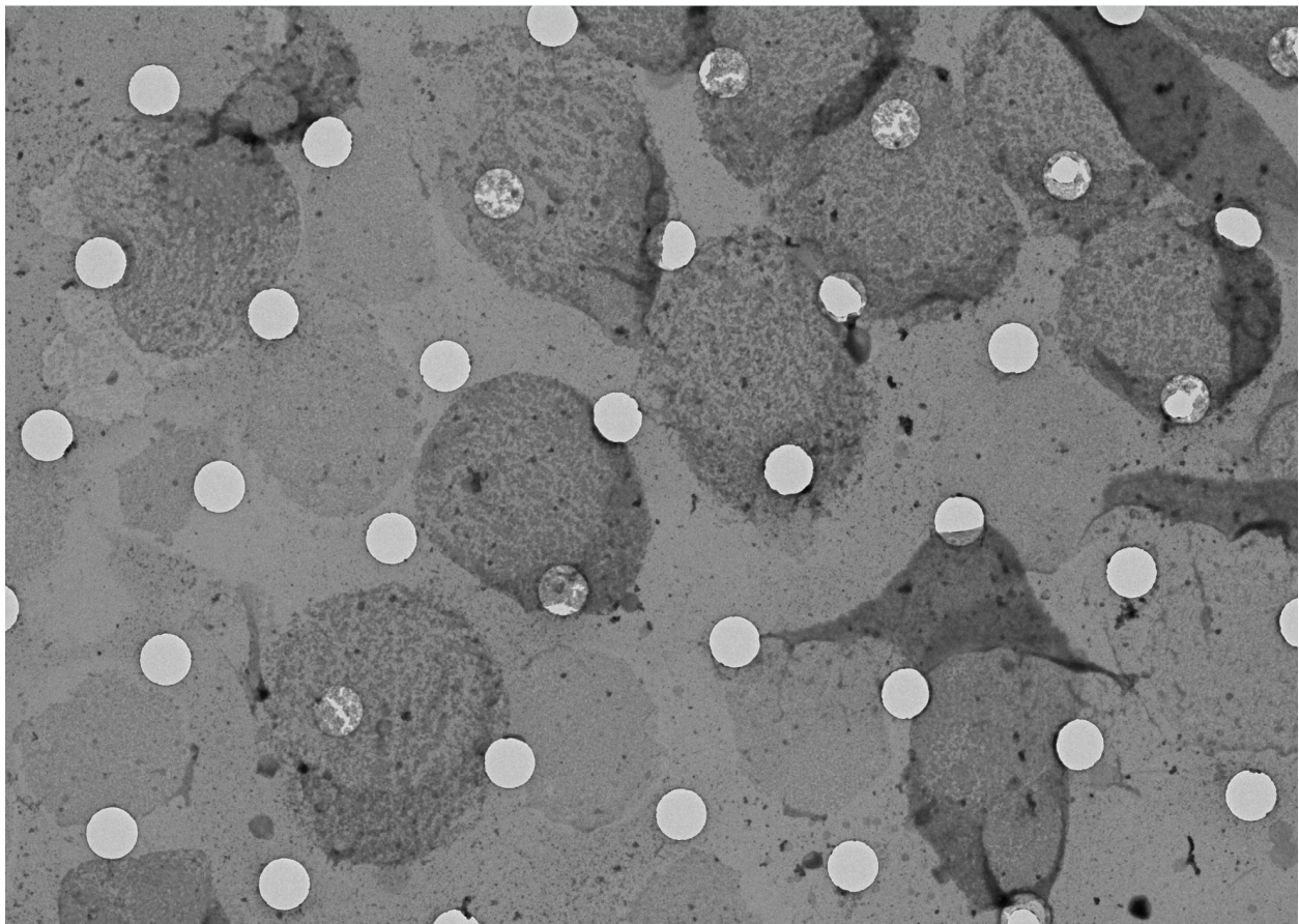
Figure 2. EM grids with negative staining of red blood cell membranes. The holes are 1 μm in diameter and 4 μm apart.
