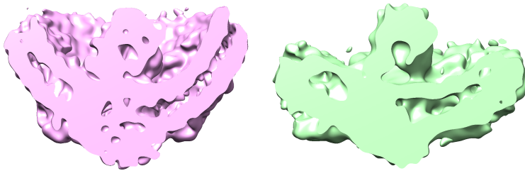
Cross-section view of Piezo1 structure solved from small and large liposomes. Maps are low-passed to 15Å.
