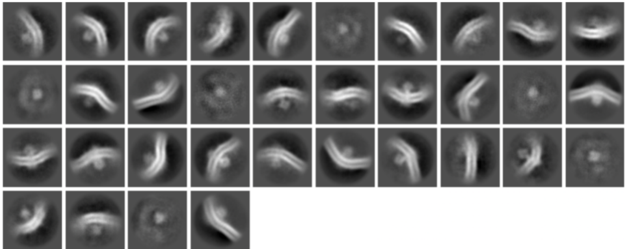
2D classification results for Piezo1 in big liposomes. Piezo1 is less curved.
