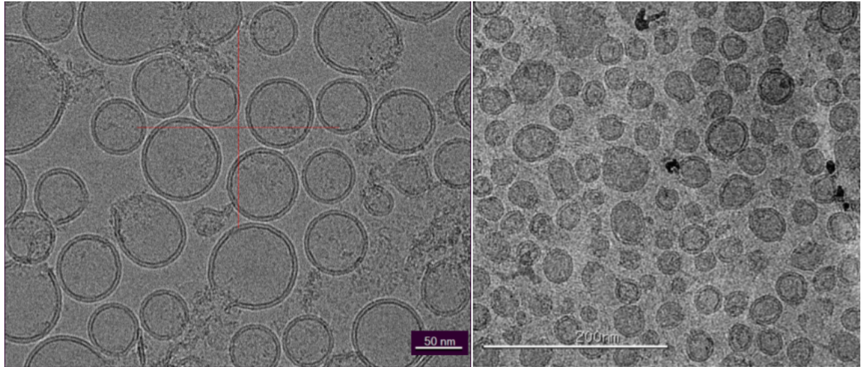
Representative micrographs of Piezo1 reconstituted in large(left) and small (right) liposomes.
