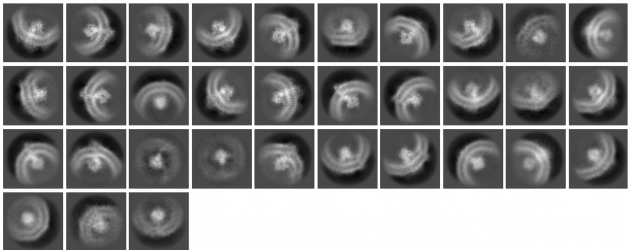
2D classification results for Piezo1 in small liposomes
