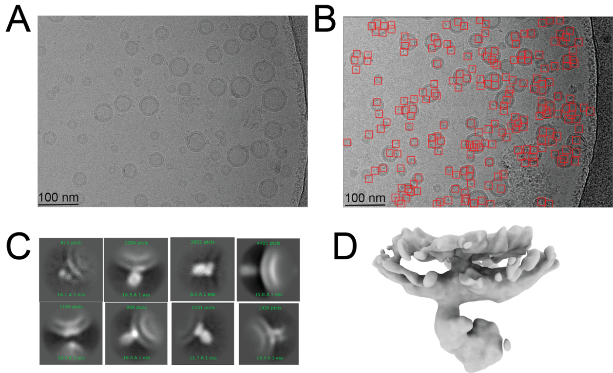
Figure 1: Feasibility of structure determination of PLC \beta -G \beta\gamma complex bound to liposomes. A: Representative micrograph of PLC \beta bound to vesicles. B: Representative micrograph from the same dataset showing particles picked by crYOLO, highlighting selective picking of PLC \beta on liposomes. C: Representative 2D classes of PLC \beta bound to liposomes from particles picked in B, box size 223 Å. D: initial reconstruction of PLC \beta bound to liposomes.
