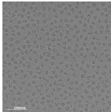
U1391C + spectinomycin
