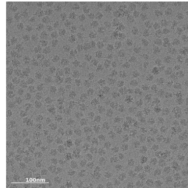
Wild type + mRNA/tRNAs
