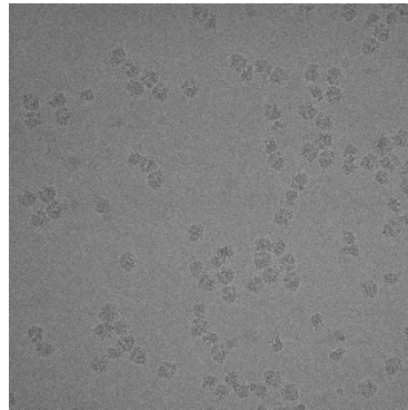
A1394G +mRNA/tRNAs (Chameleon)
