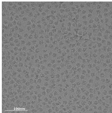
U1391C apo
