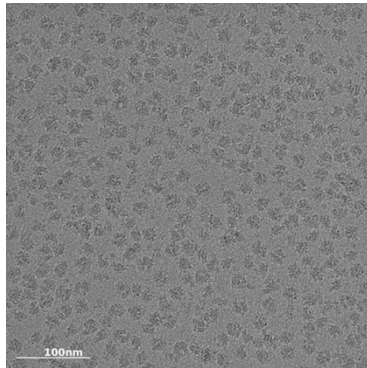
A1394G + spectinomycin
