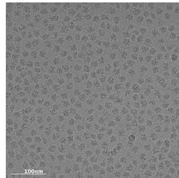
U1391C + mRNA/tRNAs
