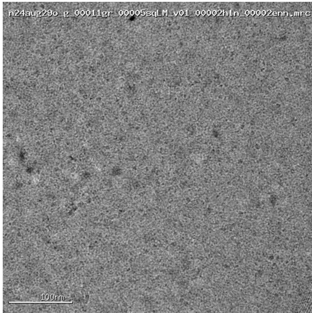
Figure 4. Representative Micrograph of Grid B3G4 Blotted with eIF3a-RP/HuR Complex Using Glacios at NCCAT (August 2024)
