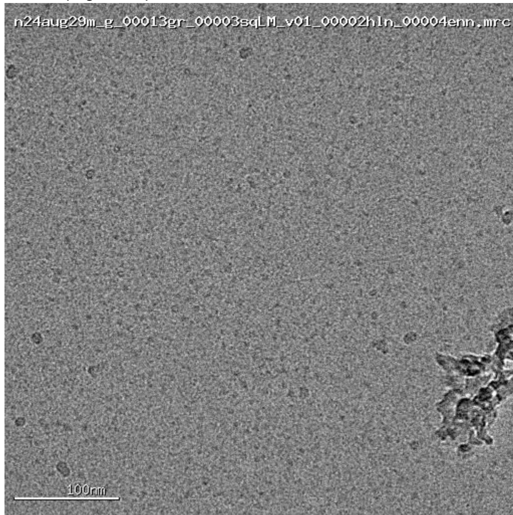
Figure 2. Representative Micrograph of Grid B3G2 Blotted with eIF3a-RP/HuR Complex Using Glacios at NCCAT (August 2024)
