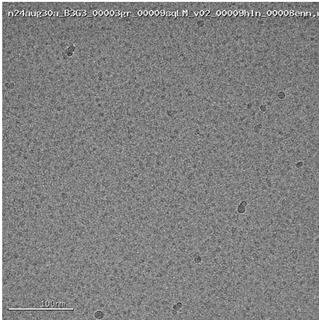
Figure 3. Representative Micrograph of Grid B3G3 Blotted with eIF3a-RP/HuR Complex Using Glacios at NCCAT (August 2024)
