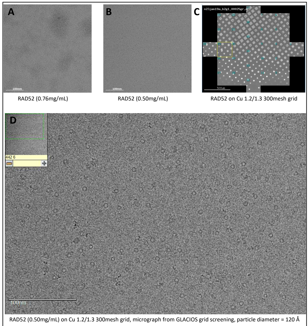
Figure 1: RAD52 micrograph from GLACIOS grid screening varying protein concentration based on the particle density. For full data collection, RAD52 protein at 0.5mg/ml was plunged frozen onto Cu 1.2/1.3 300 mesh carbon grids, screened, and stored in liquid nitrogen.
