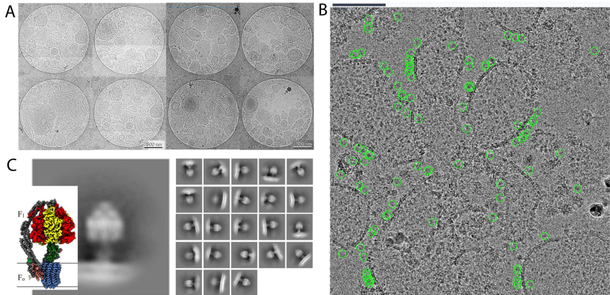
Figure: (A) Low-magnification image showing the well-distributed sub-mitochondrial particles within holes. (B) High-magnification micrograph of mitochondrial membranes, with green circles indicating regions where ATP synthase side views were detected and subsequently used for 2D classification and averaging. (C) Representative 2D class averages of ATP synthase, alongside a cartoon depiction of the previously determined ATP synthase cryo-EM structure, highlighting the structural similarity.
