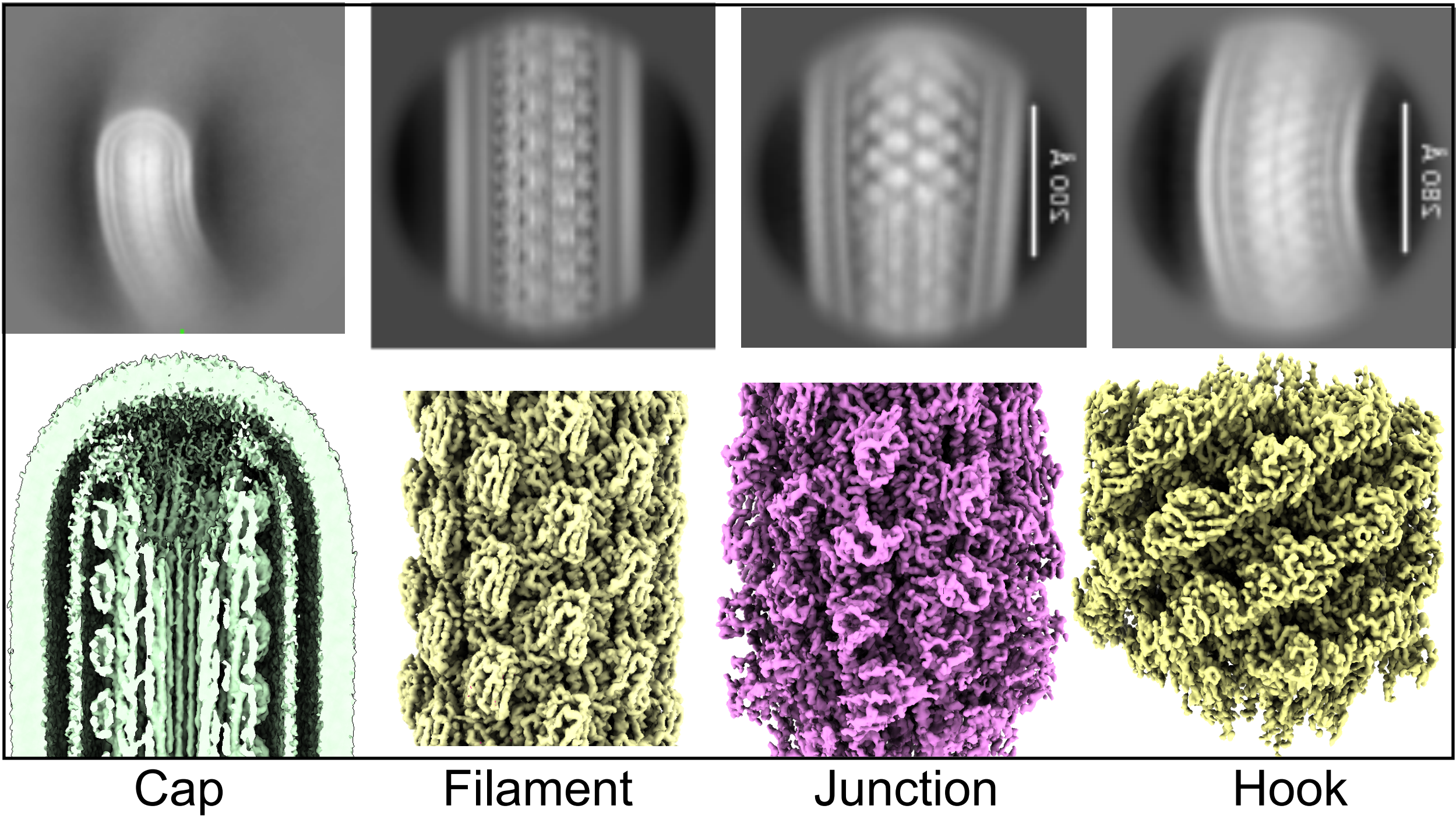
Flagellar motor
