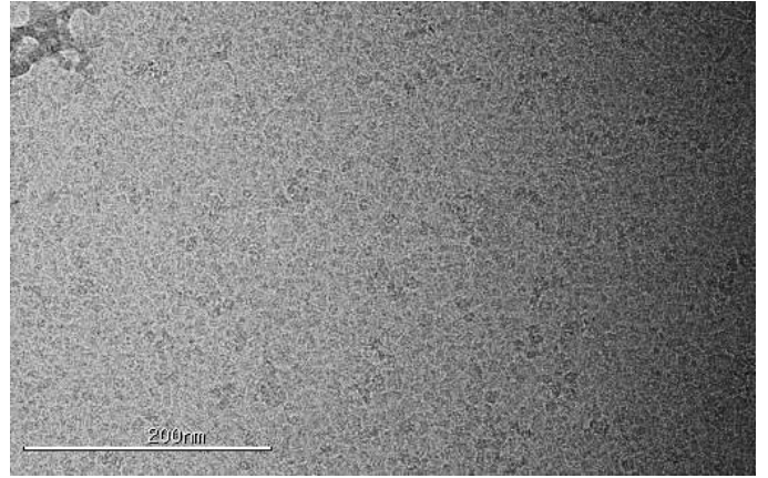
Figure 1. Representative cryo-EM micrographs of purified ATP synthase from brine shrimp ( A. ) and fruit fly ( B. ) on thin-carbon (2 mm) quantifoil grids showing the homogeneity of the purified sample.
