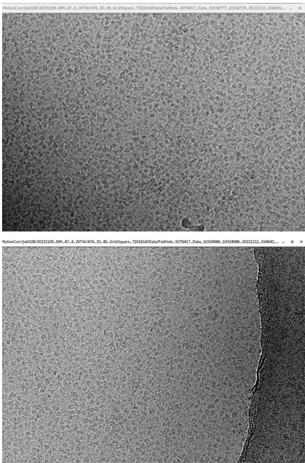
Figure 1. Representative cryo-EM micrographs of purified ATP synthase from brine shrimp on thin-carbon (2 mm) quantifoil grids showing the homogeneity of the purified sample.
