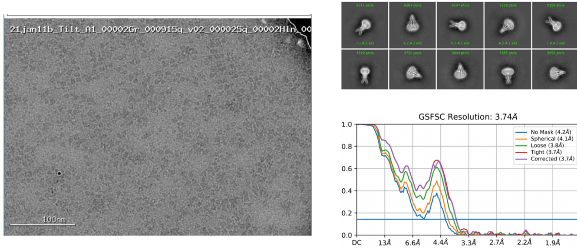
Figure 1. Example micrograph, 2D classes, and fsc curve for a mammalian Tweety homolog channel reconstituted in lipid nanodisc.
