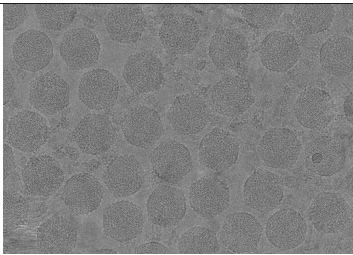
CUS-3 phages
