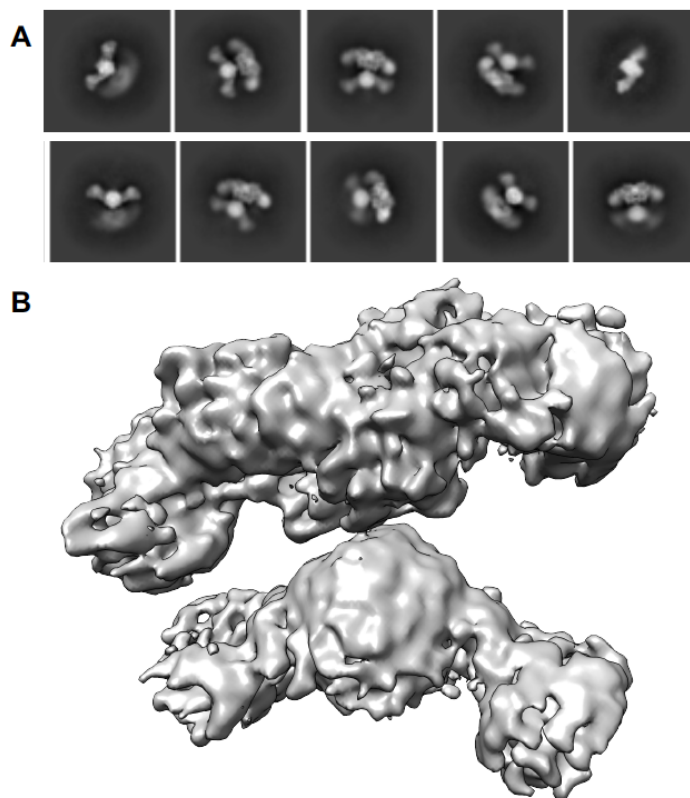
Figure 1. Preliminary cryo-EM reconstruction of a FASN/acetyl-CoA complex. (A) 2-D class averages (B) 3-D model to \sim 7\text{\AA} resolution.
