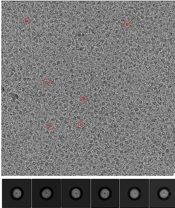
Figure1. Preliminary cryo-EM sample screening and reconstruction for Orai1 sample. Representative micrograph (top; defocus -2.5\ \mu\text{m} and 1.08\ \text{\AA}/\text{pixel} ) and 2D classification images (bottom) of mammalian Orai1. Red circles indicate examples of individual protein particles.
