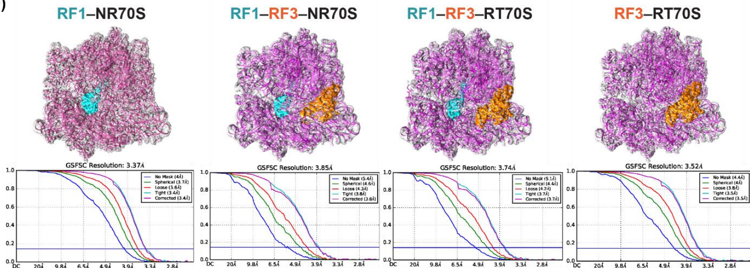
Figure: (A) Sample single-molecule fluorescence trace showing four different compositional/conformational states of the ribosome during translation termination (B) Schematic of the pathway of translation termination highlighting a proposed conformational switch before RF3-mediated ribosome rotation (C) Particle image and 2D Classification of the preliminary CryoEM data collection (D) EM map of the four ribosome states and their respective FSC plots
