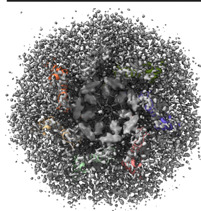
YnaI in a close state
