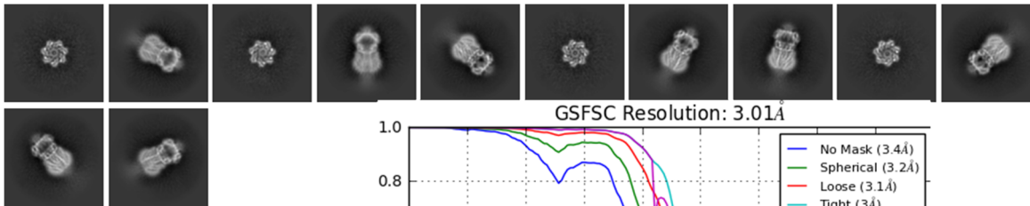
YnaI in a close state
