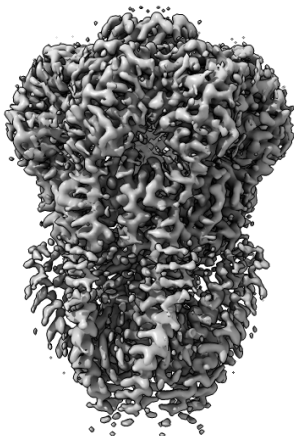
MscS in a close state
