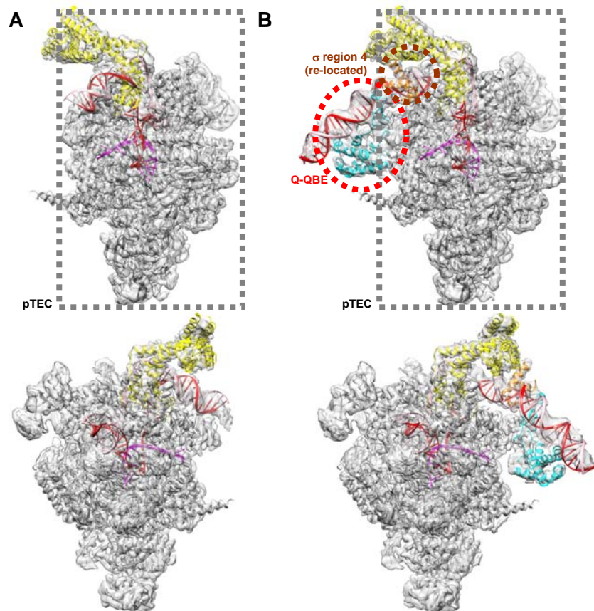
Fig. 2. Fitted maps for the two identified 3D sub-classes (two views of each). (A) Target for Qlambda loading (sigma-containing TEC paused at the PR'lambda sigma-dependent pause element; 61,000 particles; 3.4 Å). (B) Product of Qlambda loading (fully engaged Qlambda loading complex; 50,000 particles; 3.5 Å)
