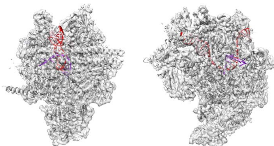
Fig. 2. Fitted map. Gray surface, cryo-EM initial reconstruction; fitted structural model of TEC paused (RNAP, DNA template strand, DNA non-template strand, and RNA from PDB 6ALF as gray, red, pink, and magenta ribbons).
