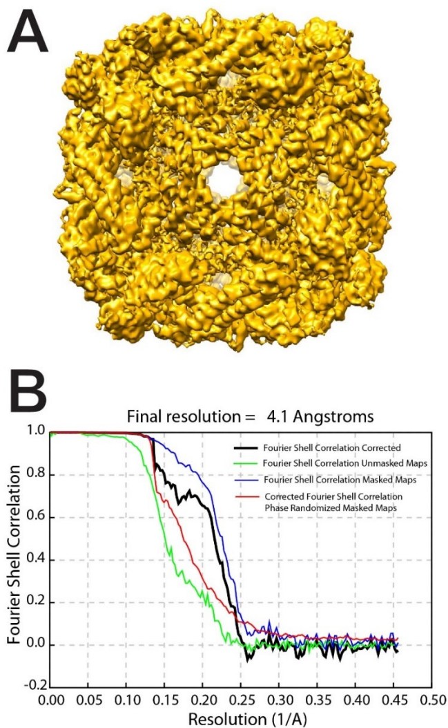
Figure S1. Cryo-electron microscopy of AbmR complex. We have processed the data collected about four weeks ago at NYSBC under NCCAT support and obtained a density map at 4.1Å resolution using Relion. (A) The density map revealed many structural details and some large side chains. (B). Gold-standard FSC demonstrates the map has reached 4.1Å resolution. Improved map resolution is needed to build an atomic model with confidence.
