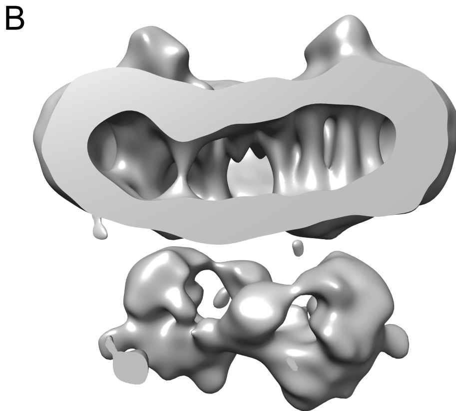
A) A representative micrograph and two-dimensional (2D) class averages of the furosemide (a diuretics) bound NKCC1. The 2D averages show clear two-fold symmetry. B) 3D cryo-EM reconstruction of NKCC1 at 8.5 Å resolution. Note, several transmembrane helices are visible in this cut-open view.
