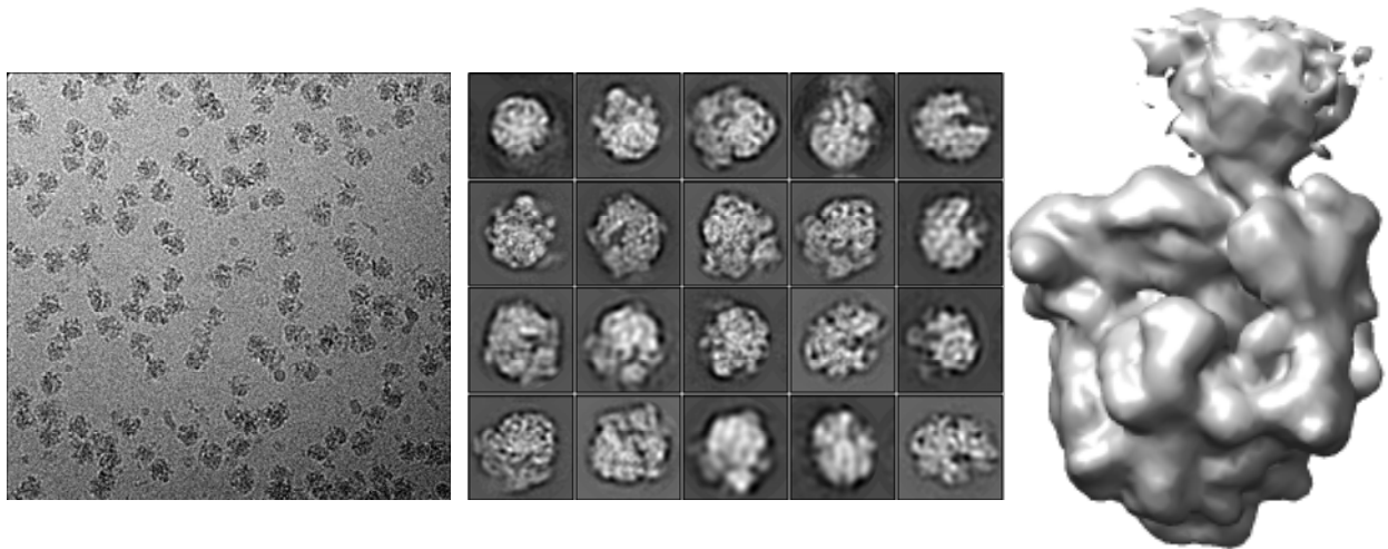
Figure 1. Expressome-1: representative micrograph, 2-D classes, and preliminary reconstruction (7.7 Å).
