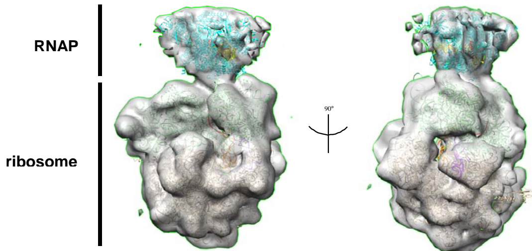
Figure 2. Expressome-1: fitted map (two orthogonal views). Gray surface, cryo-EM reconstruction (7.7 Å); density feature labelled "RNAP," fitted cryo-EM structure of transcribing RNAP (PDB 6ALH; RNAP as cyan ribbon, DNA as yellow ribbon, mRNA as red ribbon); density feature labelled "ribosome," fitted cryo-EM structure model of translating 70 S ribosome (PDB 4V6G; 30S as green ribbon; 50S as gold ribbon; tRNA as purple ribbon; mRNA as red ribbon).
