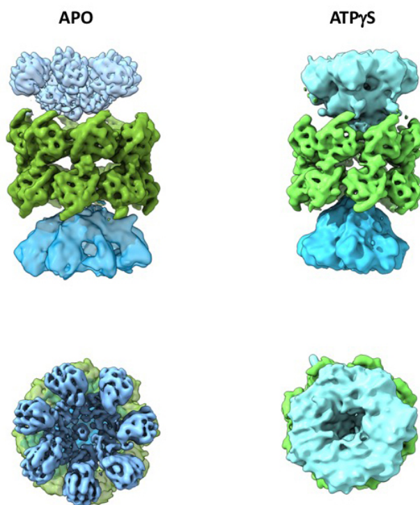
Figure 1- Comparison of apo and ATP \gamma S maps showing differences in the helicase (blue) rings. The OBD (green) rings stacked on a head to head orientation.
