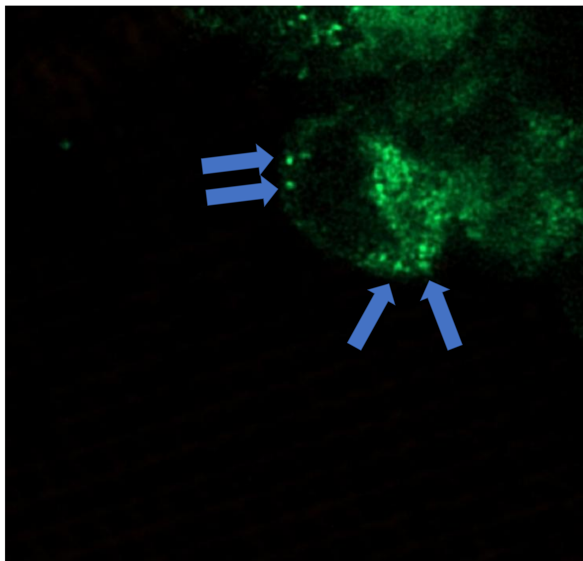
Figure 1. A) Single-particle structure of GSDMD Xia et al., Nature 2021. B) Negative stain of a bacterial GSDMD homolog organized as a net-like structure Johnson et al., bioRxiv 2021. C) FLM of frozen plunged THP-1 cells expressing fluorescent GSDMD. The blue arrows show GSDMD puncta on a thin edge membrane.
