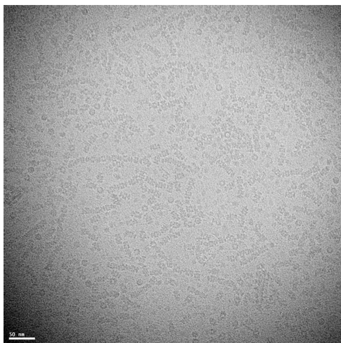
Figure 2- New grids prepared with the new truncated Rep68 protein. Image collected on a F20 with ccd camera.
