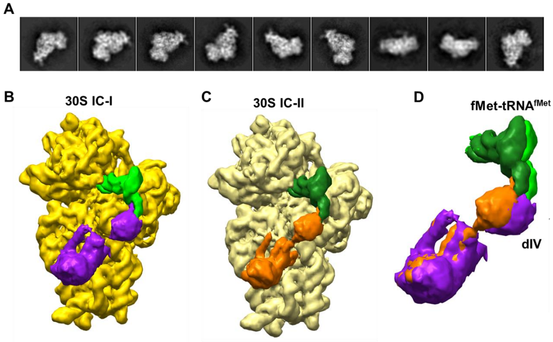
Figure: Conformations of 30S IC. (A) Representative 2D classes of the 30S ribosome. (B) & (C) Cryo-EM-derived Coulomb potential maps of 30S IC-I (5.3 Å) and 30S IC-II (5.4 Å). (D) Magnified view of Superposition of fMet-tRNA fmet and IF2 from two conformations of 30S IC.
