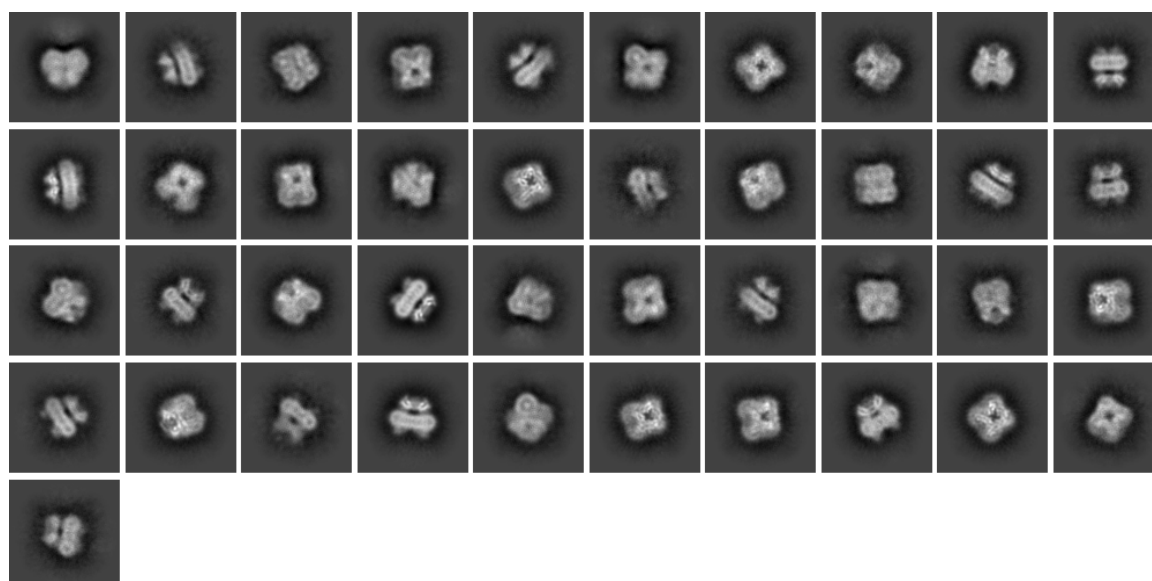
Fig. 2 Good 2D classes
