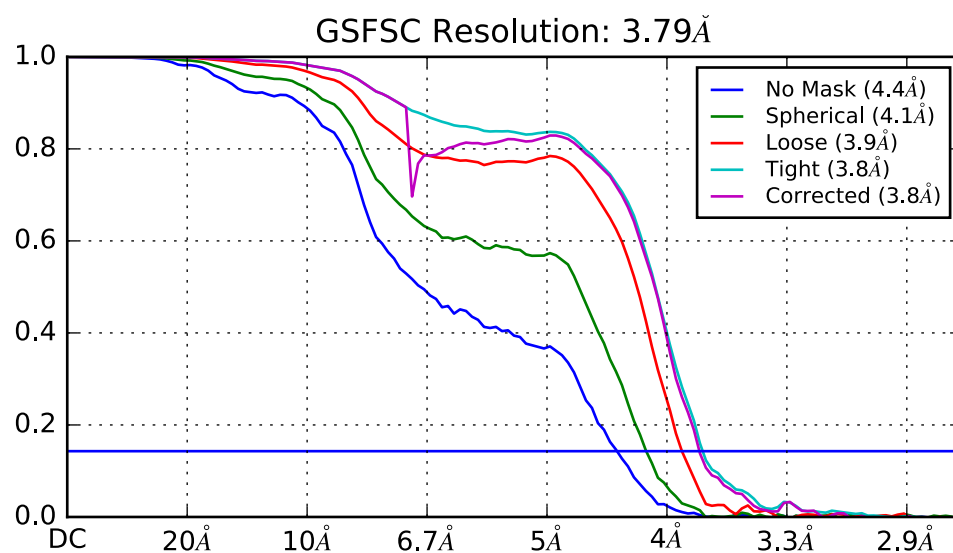
FSC curves from preliminary dataset collection from talos arctica imaged at 1.3 Å/pix, from ~600k particles and 2,400 micrographs.
