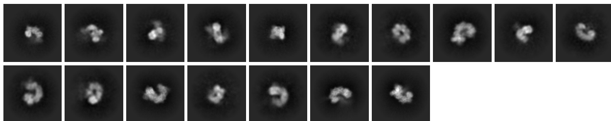
Representative cryosparc 2D class averages
