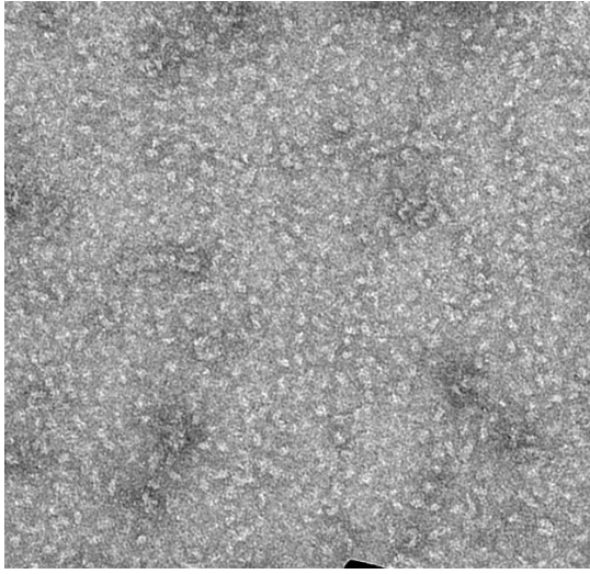
Figure 1. Negative stain images of nucleosome-B-Myb DBD complex reconstructed with the Widom 601 positioning sequence.
