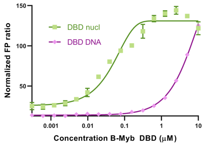
Figure 2. Fluorescence polarization assay showing affinity of B-Myb DBD to nucleosomes and DNA. B-Myb DBD binds to nucleosomes with affinity of 50 \pm 1.5 nM and free DNA with 5 \pm 0.05 μM.
